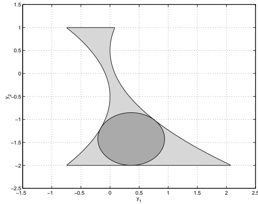
Figure 1.1. A disk with maximal area in a nonconvex container
