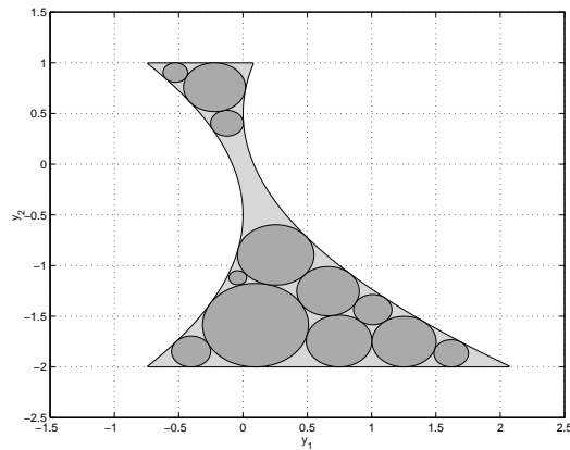
Figure 1.2. Twelve disks with maximal total area in a nonconvex container
